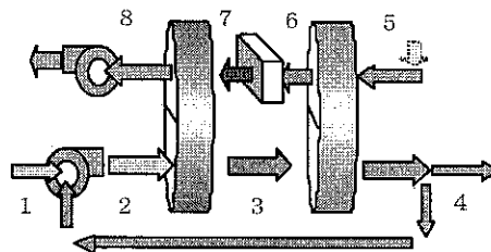
Fig.9 Circulation Processing System
