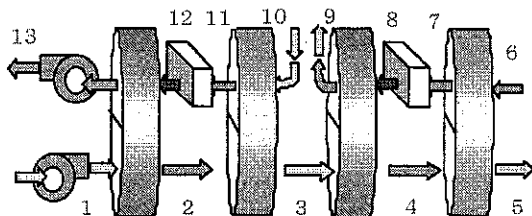
Fig.7 Double Staged Desiccant Air-conditioning System
